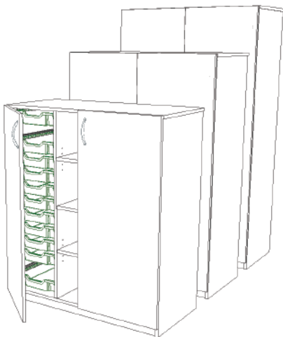
D. Tall tray stock cupboard
