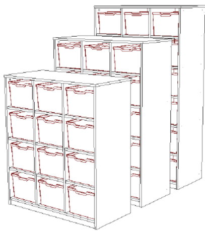
H. Tall extra deep tray unit
