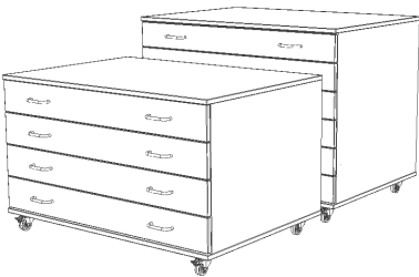
K. Mobile A1 plan chest 1021(W) x 710(D)mm 620(H) 4 drawer EVS005A ** £277.75 790(H) 6 drawer EVS005B ** £363.75
