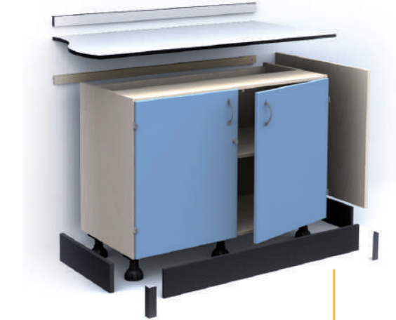
Moisture resistant plinth
